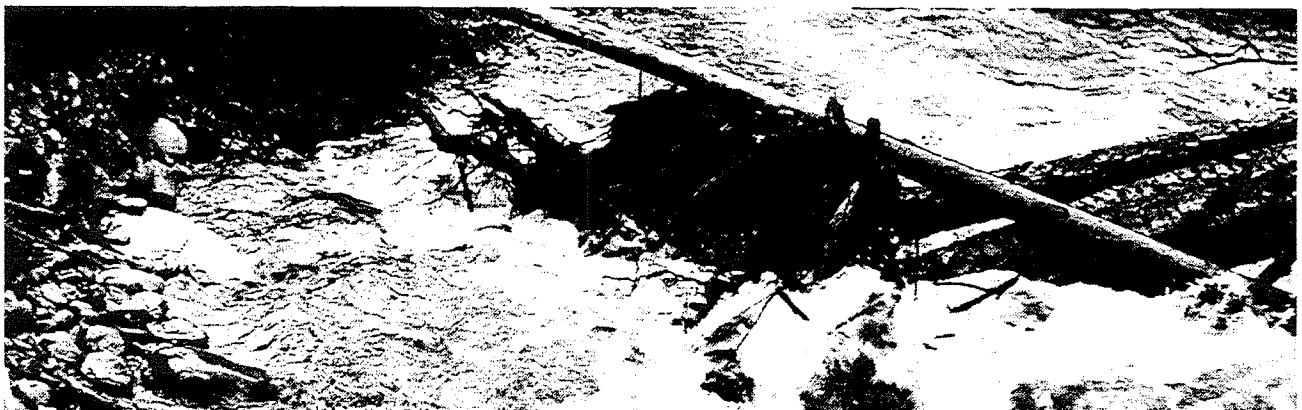
Overtured shoreline trees become obstructions and flow deflectors as shown here. If frequent in the reach, rate this item "Poor".
