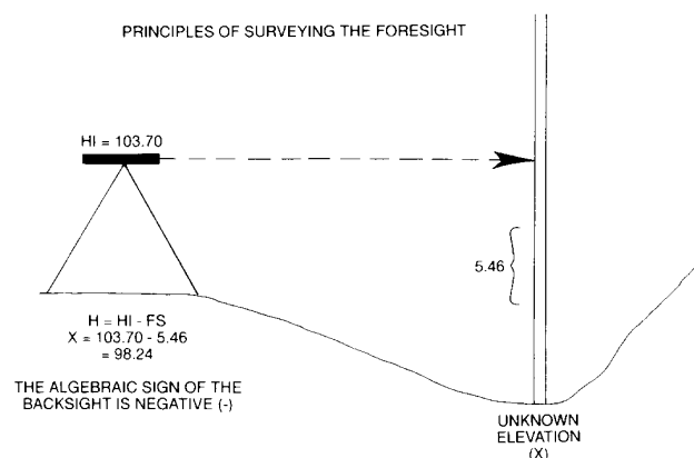
Figure 27. Surveying the foresight.
