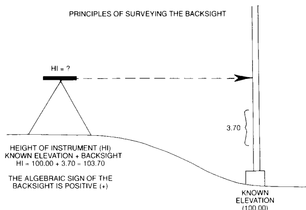
Figure 26. Surveying the backsight.
