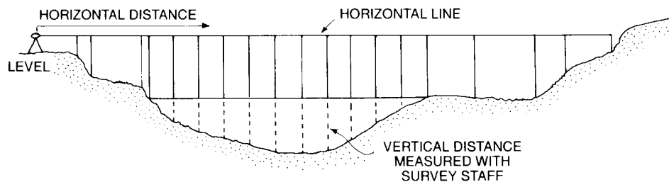
Figure 31. Diagram of a cross-section survey.
