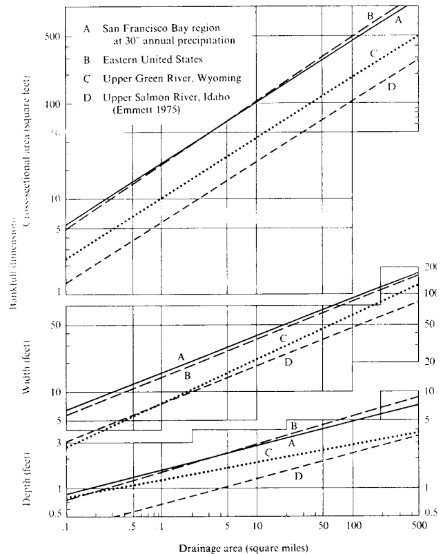
Figure 46. Average values of bankfull channel dimensions as functions of drainage area for four regions. From: Water In Environmental Planning by Thomas Dunne and Luna B. Leopold. Copyright © 1978 by W.H. Freeman and Company. Reprinted with permission.
